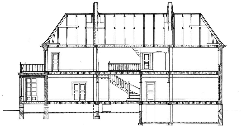
Skärning C-D.
